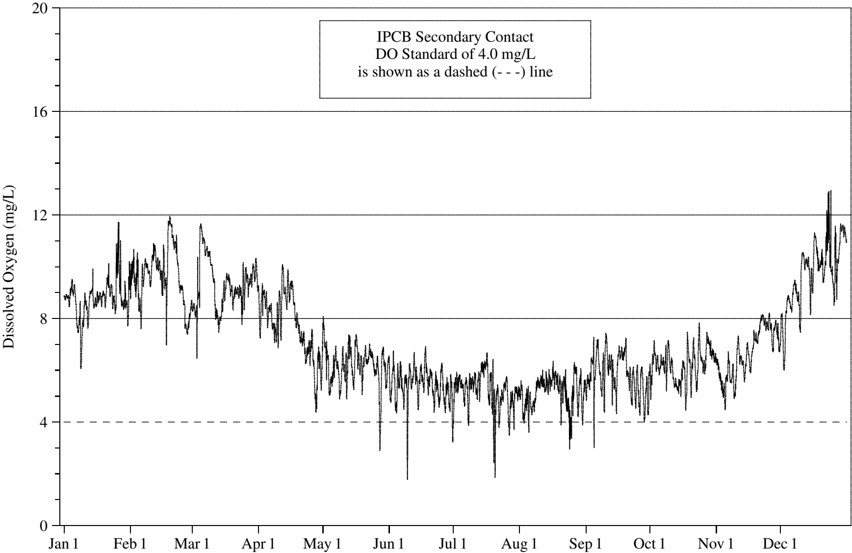
FIGURE 6: DISSOLVED OXYGEN CONCENTRATION MEASURED HOURLY AT KINZIE STREET ON THE NORTH BRANCH CHICAGO RIVER FROM JANUARY 1, 2008 THROUGH DECEMBER 31, 2008
